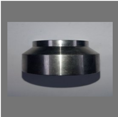
Gi Coupling
